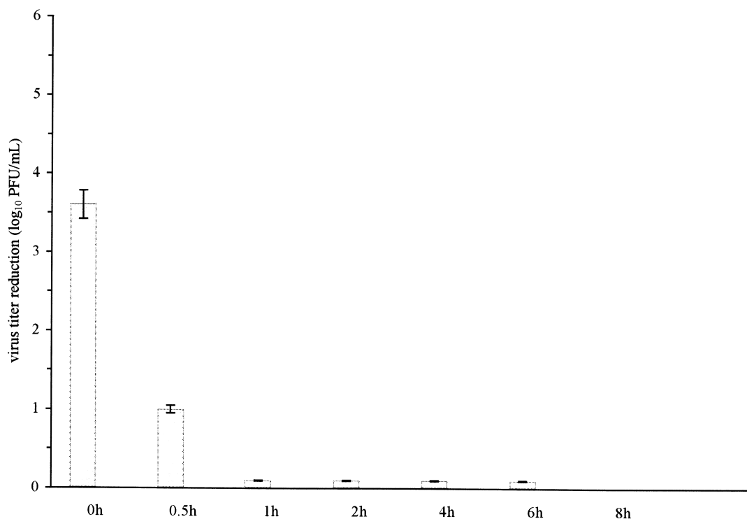
Figure 1. Effect of time of 9a (10 \mu M) addition on virus inhibition from single-round replication of polio 1. Time 0 = post 2 h absorption period at 4 °C. All values are mean \pm S.D. of three separate assays.
