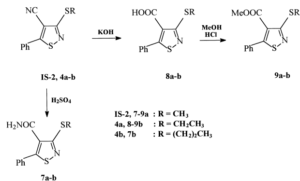
Scheme 2. Synthesis of compounds 7a,b , 8a,b and 9a,b .
